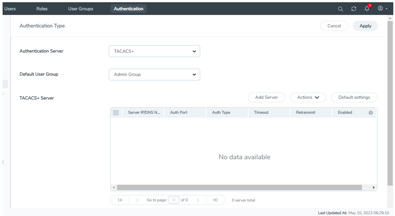
Figure 3 TACACS+ Page
