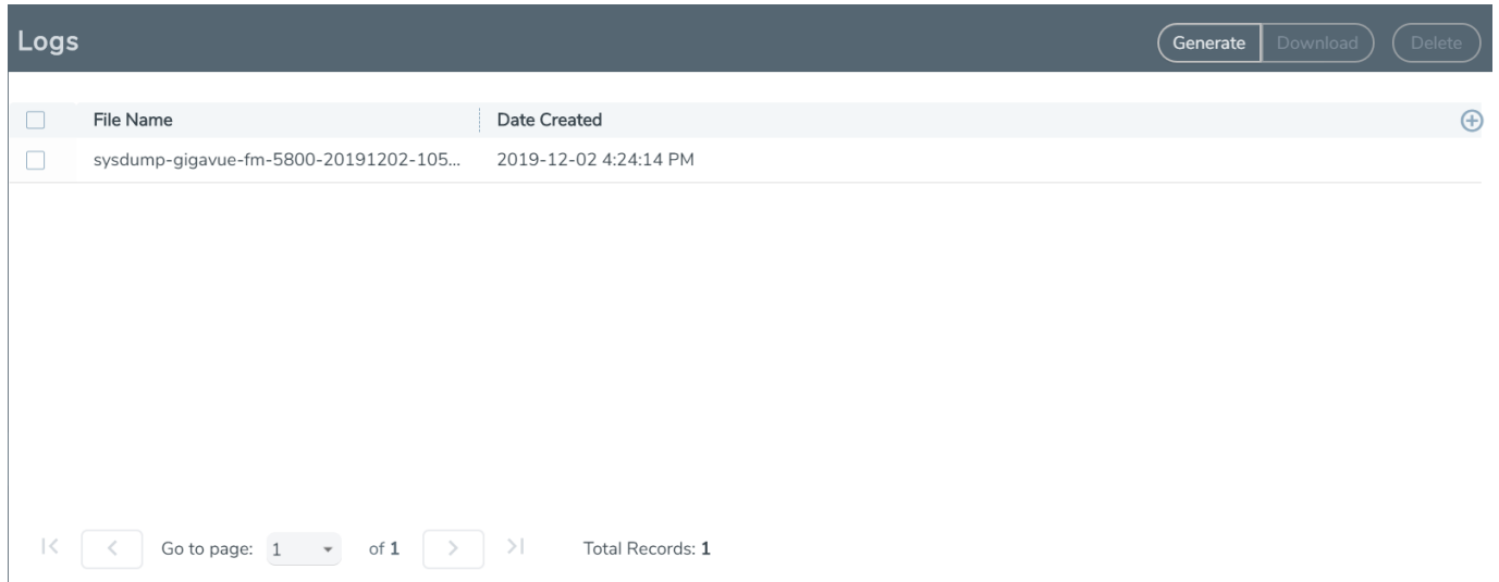
Figure 21 Logs Page
